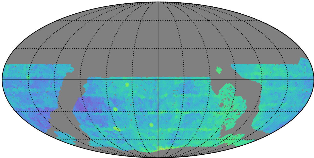
roll_pause_mjdp270_v3.4_10yrs WFD r band: Median Season Length
