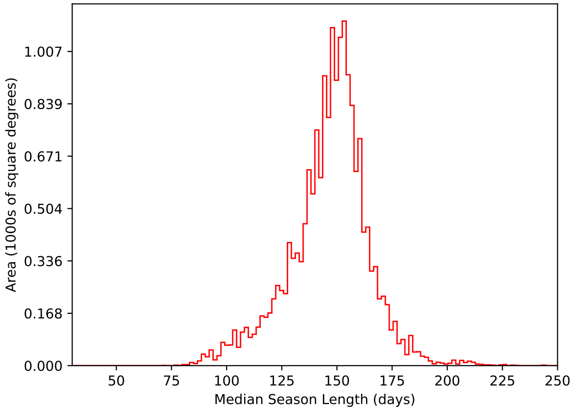
roll_pause_mjdp270_v3.4_10yrs WFD i band: Median Season Length
