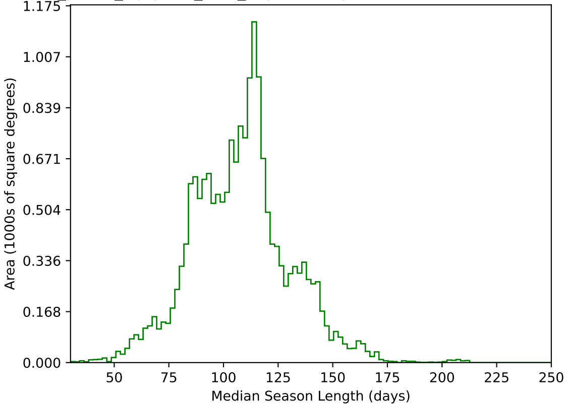
roll_pause_mjdp270_v3.4_10yrs WFD g band: Median Season Length
