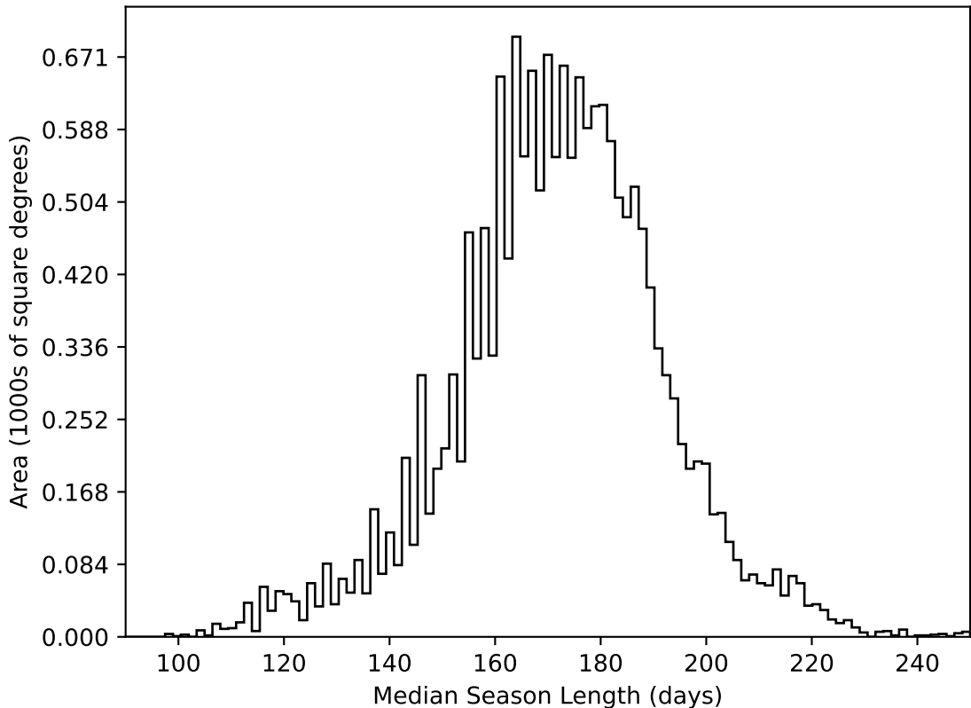
roll_pause_mjdp270_v3.4_10yrs WFD all bands: Median Season Length
