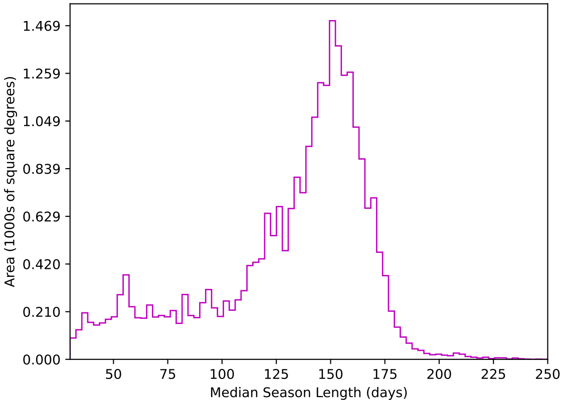
roll_pause_mjdp270_v3.4_10yrs All sky z band: Median Season Length
