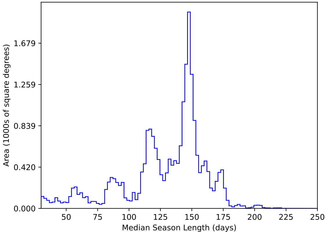
roll_pause_mjdp270_v3.4_10yrs All sky y band: Median Season Length
