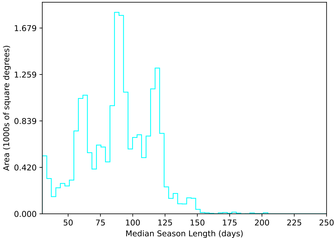
roll_pause_mjdp270_v3.4_10yrs All sky u band: Median Season Length
