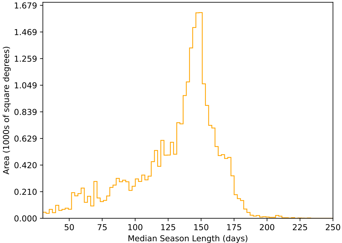
roll_pause_mjdp270_v3.4_10yrs All sky r band: Median Season Length
