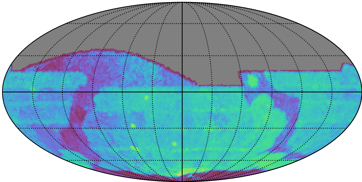
roll_pause_mjdp270_v3.4_10yrs All sky i band: Median Season Length
