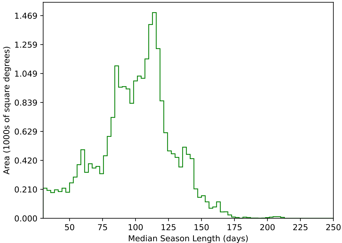
roll_pause_mjdp270_v3.4_10yrs All sky g band: Median Season Length
