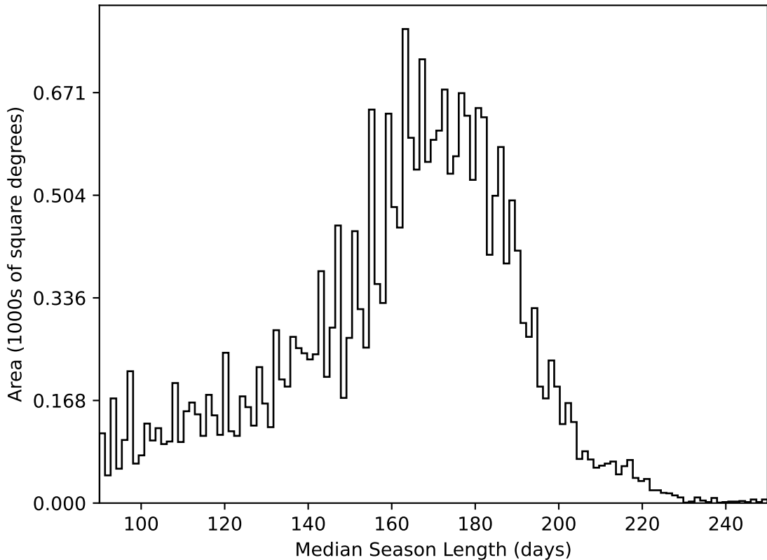
roll_pause_mjdp270_v3.4_10yrs All sky all bands: Median Season Length
