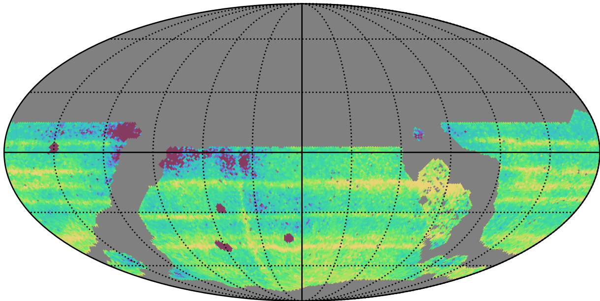
roll_pause_mjdp270_v3.4_10yrs WFD: Median Intra-Night Gap
