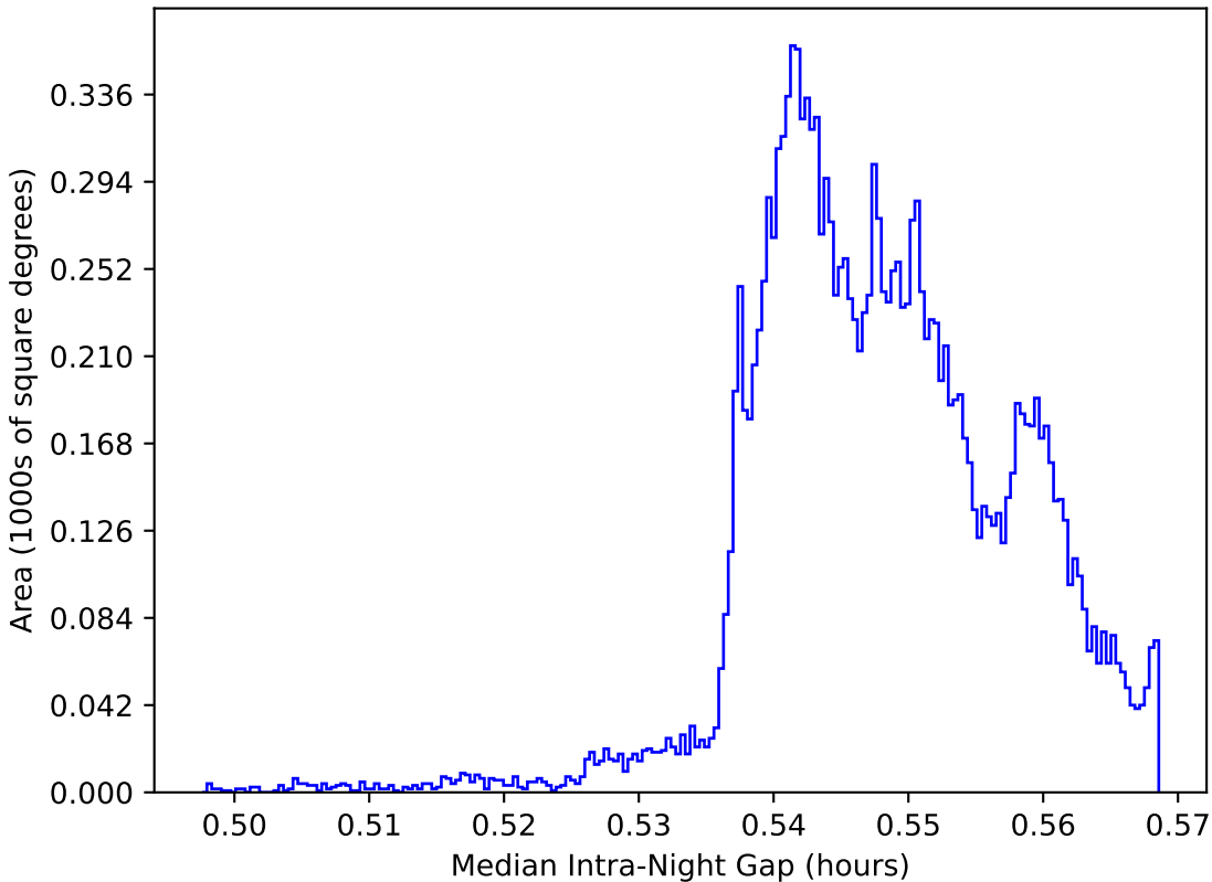
roll_pause_mjdp270_v3.4_10yrs WFD: Median Intra-Night Gap
