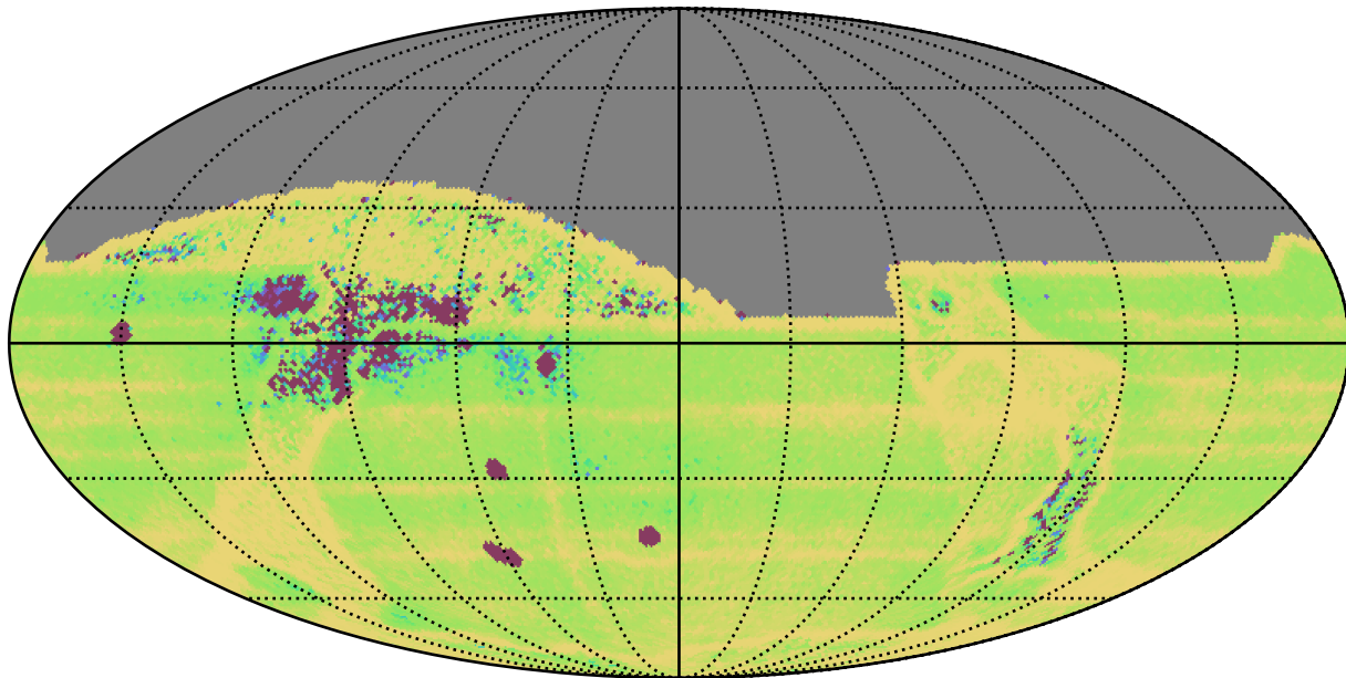
roll_pause_mjdp270_v3.4_10yrs All sky: Median Intra-Night Gap
