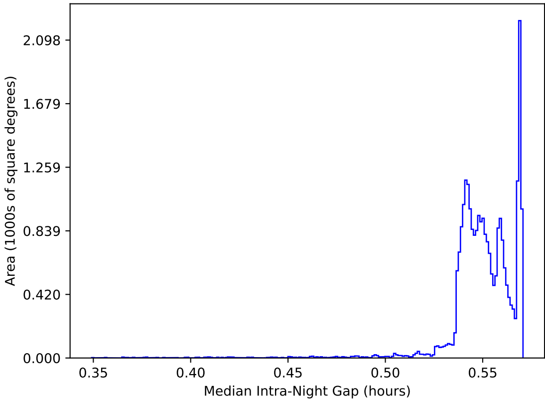
roll_pause_mjdp270_v3.4_10yrs All sky: Median Intra-Night Gap
