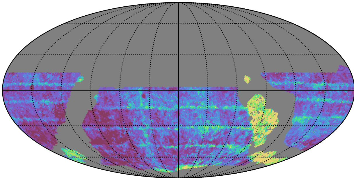
roll_pause_mjdp270_v3.4_10yrs WFD z band: Median Inter-Night Gap
