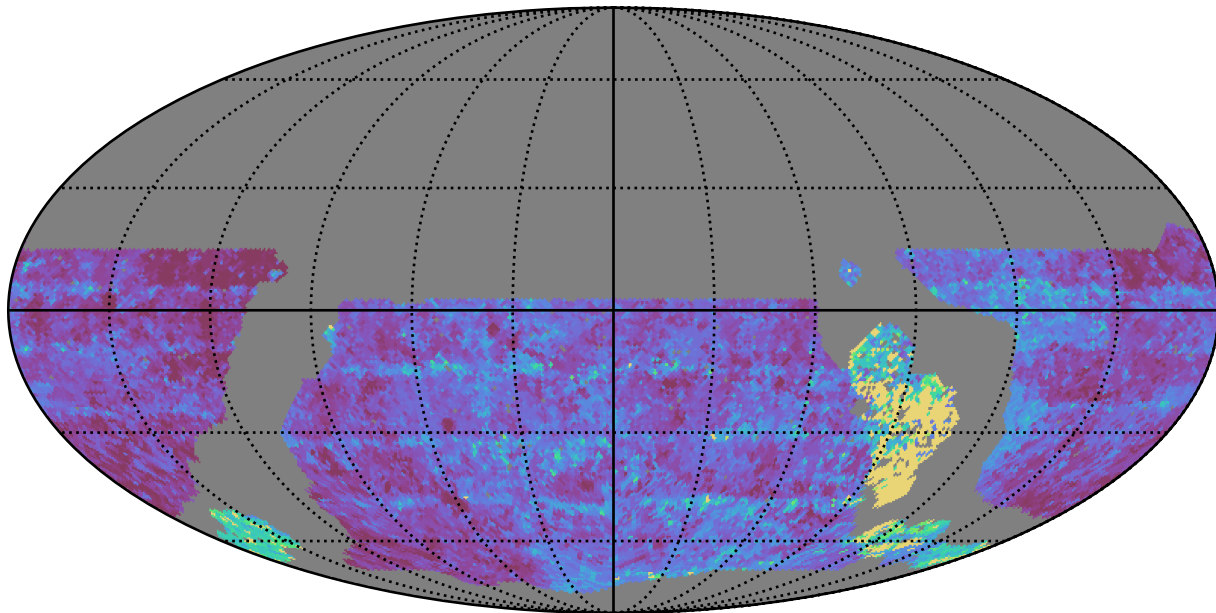
roll_pause_mjdp270_v3.4_10yrs WFD u band: Median Inter-Night Gap
