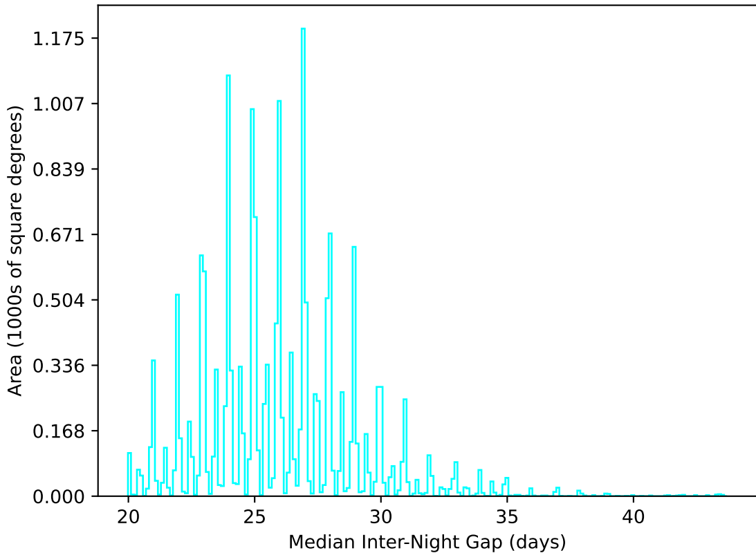
roll_pause_mjdp270_v3.4_10yrs WFD u band: Median Inter-Night Gap
