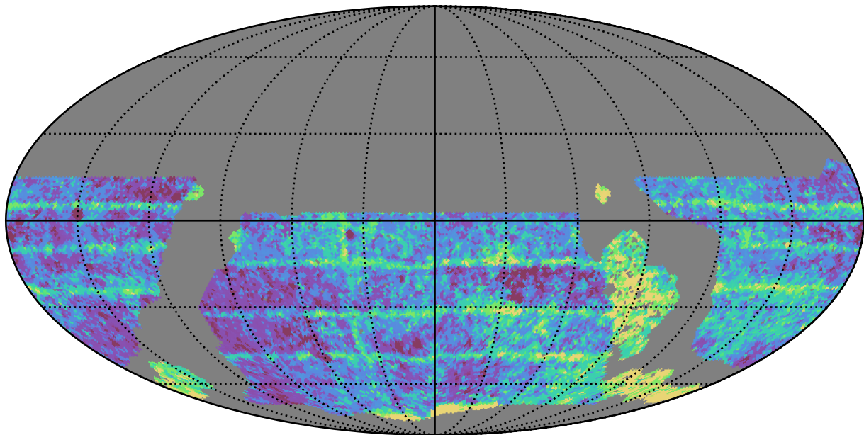
roll_pause_mjdp270_v3.4_10yrs WFD i band: Median Inter-Night Gap
