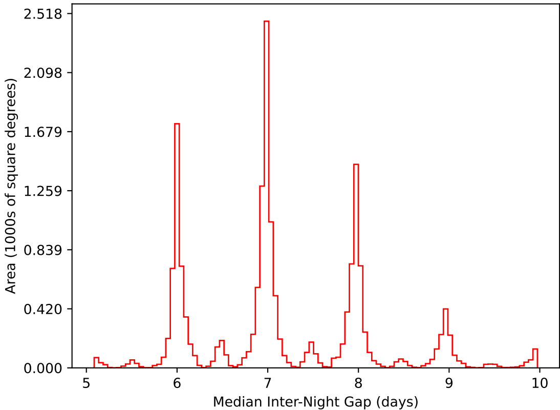
roll_pause_mjdp270_v3.4_10yrs WFD i band: Median Inter-Night Gap
