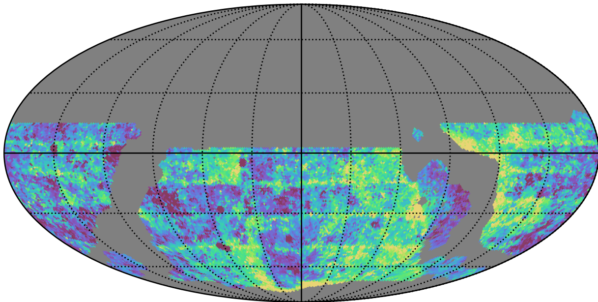
roll_pause_mjdp270_v3.4_10yrs WFD g band: Median Inter-Night Gap
