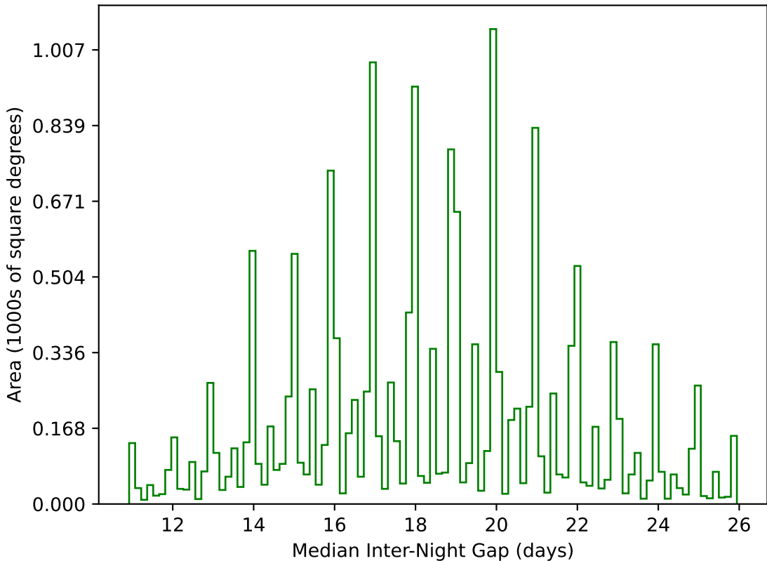
roll_pause_mjdp270_v3.4_10yrs WFD g band: Median Inter-Night Gap
