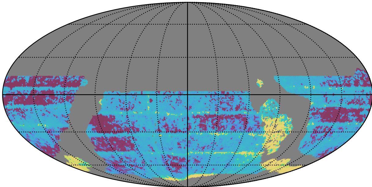
roll_pause_mjdp270_v3.4_10yrs WFD all bands: Median Inter-Night Gap
