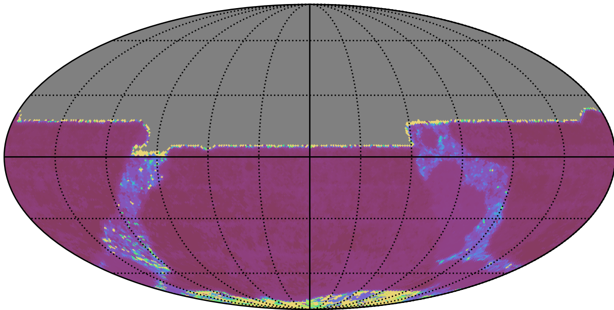
roll_pause_mjdp270_v3.4_10yrs All sky y band: Median Inter-Night Gap
