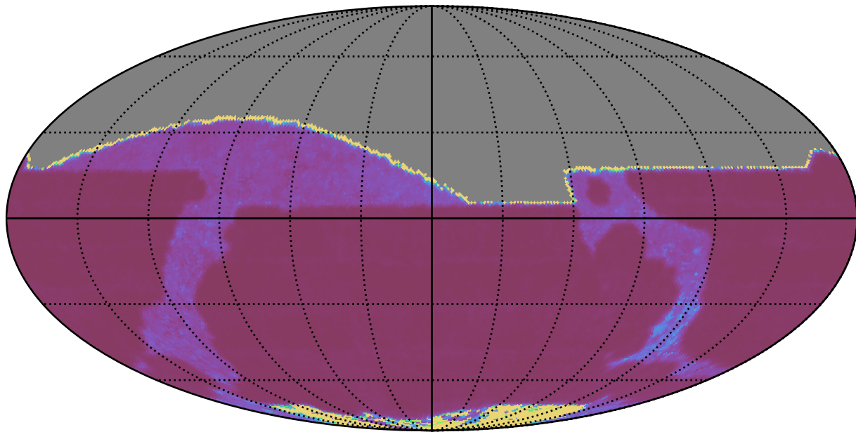
roll_pause_mjdp270_v3.4_10yrs All sky r band: Median Inter-Night Gap
