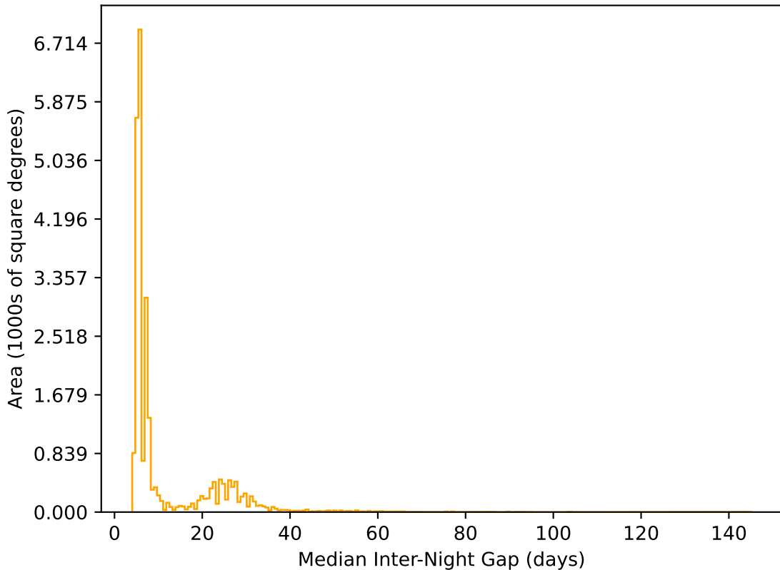
roll_pause_mjdp270_v3.4_10yrs All sky r band: Median Inter-Night Gap
