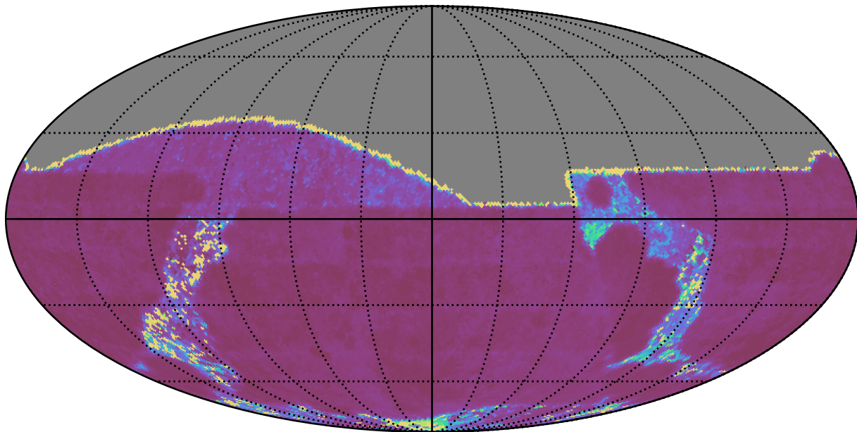
roll_pause_mjdp270_v3.4_10yrs All sky g band: Median Inter-Night Gap
