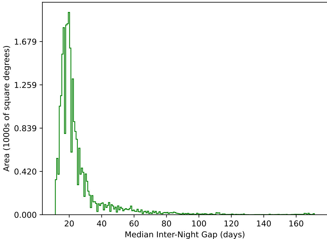
roll_pause_mjdp270_v3.4_10yrs All sky g band: Median Inter-Night Gap
