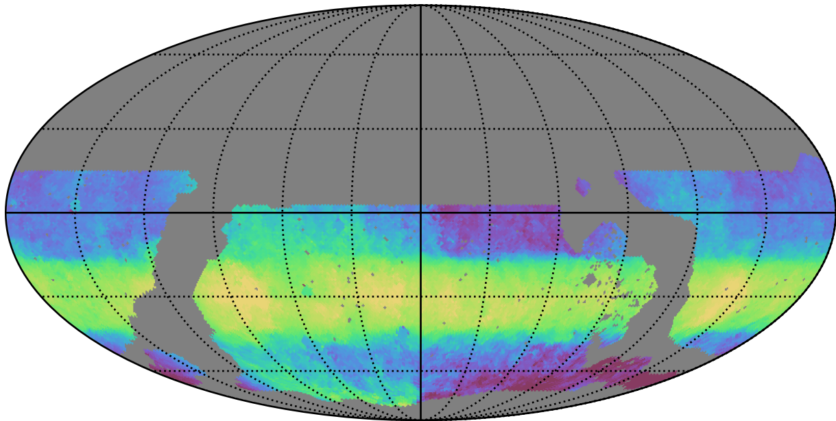
roll_pause_mjdp270_v3.4_10yrs WFD z band: Median HA
