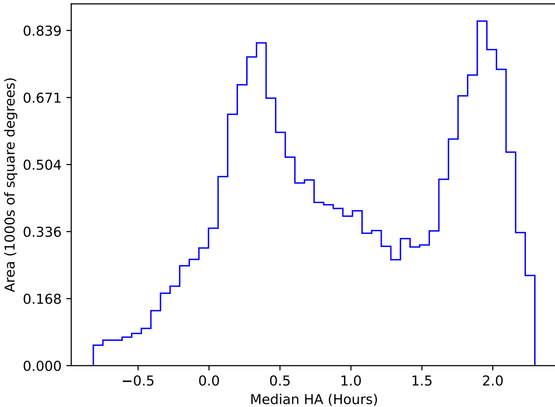
roll_pause_mjdp270_v3.4_10yrs WFD z band: Median HA
