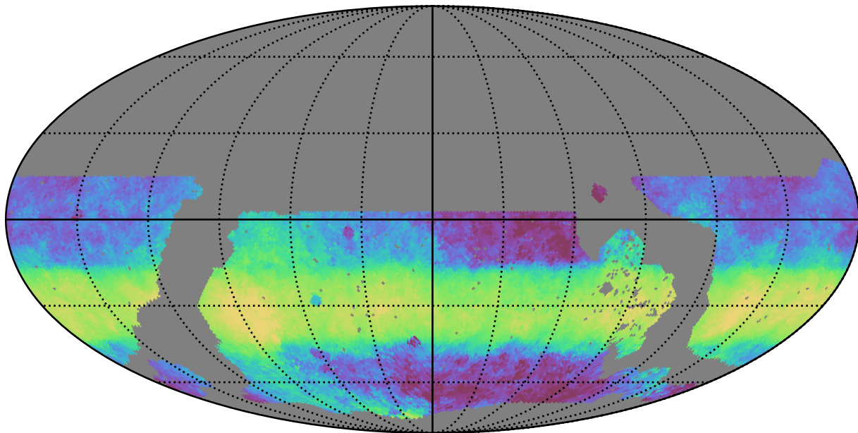
roll_pause_mjdp270_v3.4_10yrs WFD y band: Median HA
