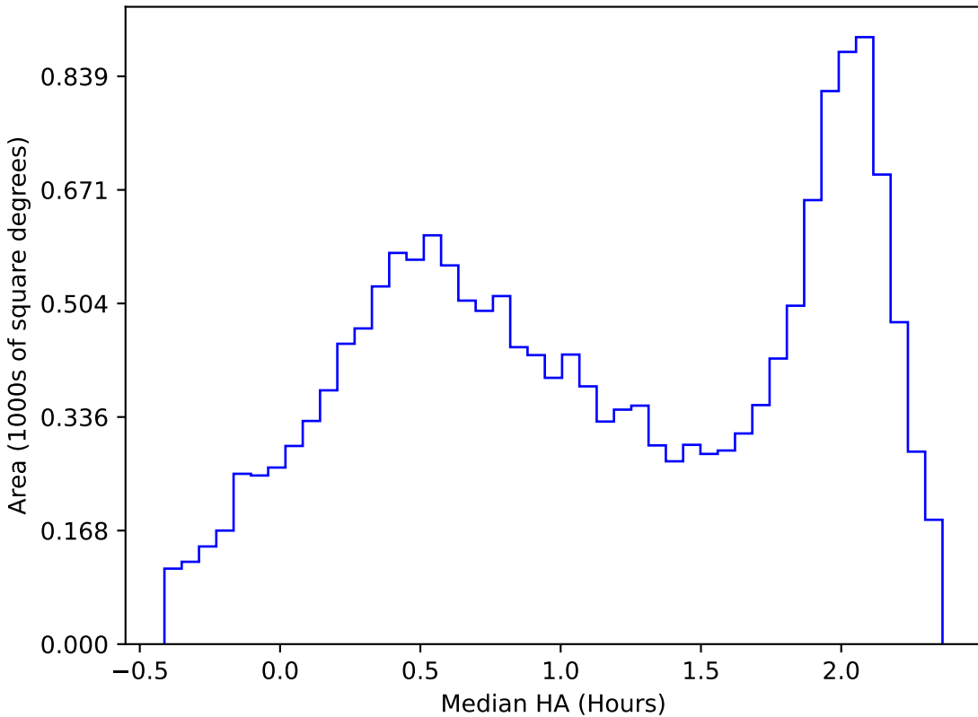
roll_pause_mjdp270_v3.4_10yrs WFD y band: Median HA
