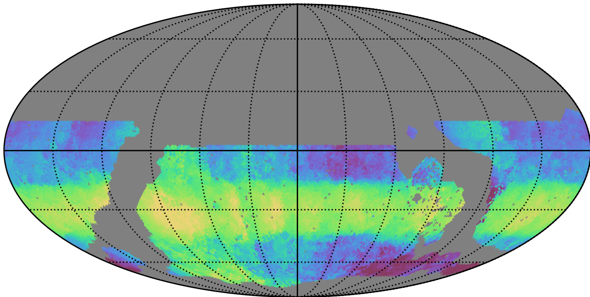
roll_pause_mjdp270_v3.4_10yrs WFD u band: Median HA
