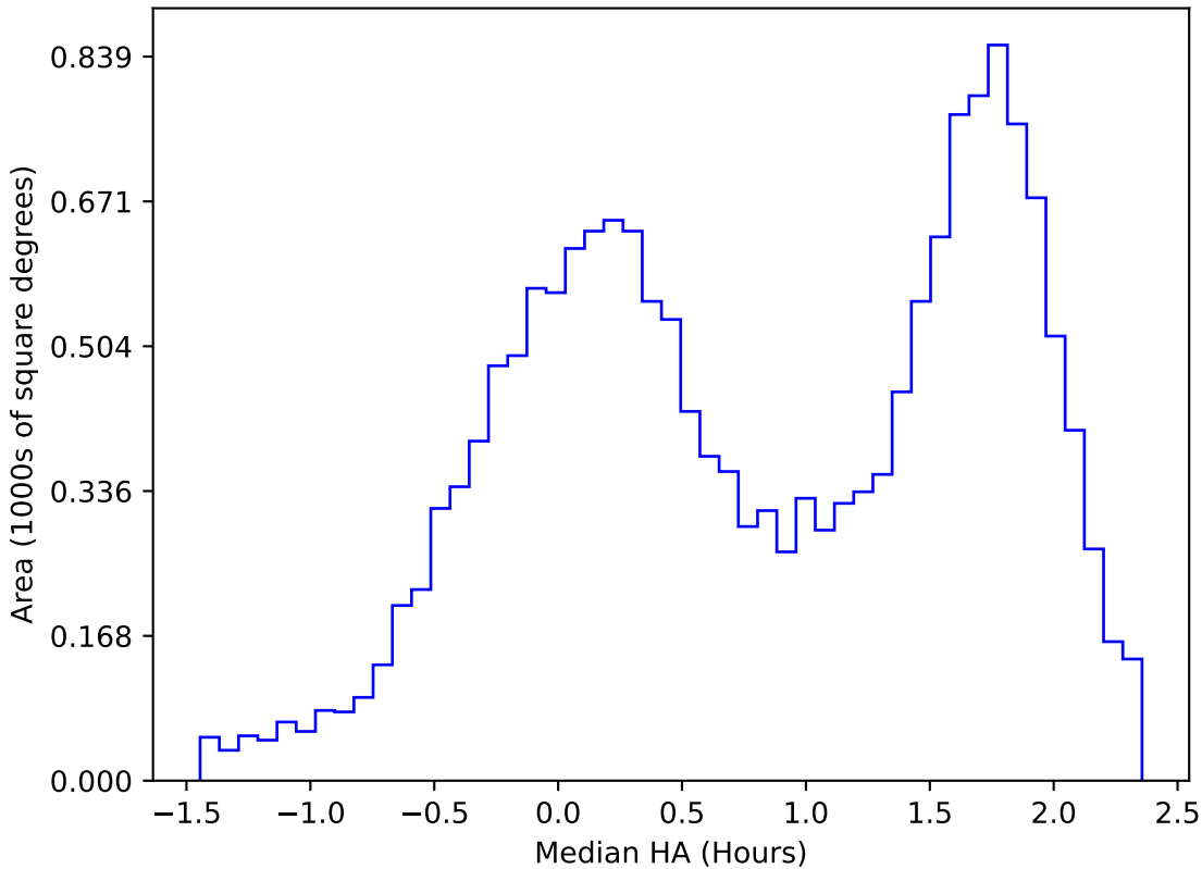
roll_pause_mjdp270_v3.4_10yrs WFD u band: Median HA
