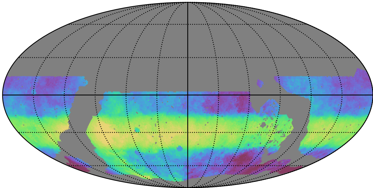
roll_pause_mjdp270_v3.4_10yrs WFD r band: Median HA
