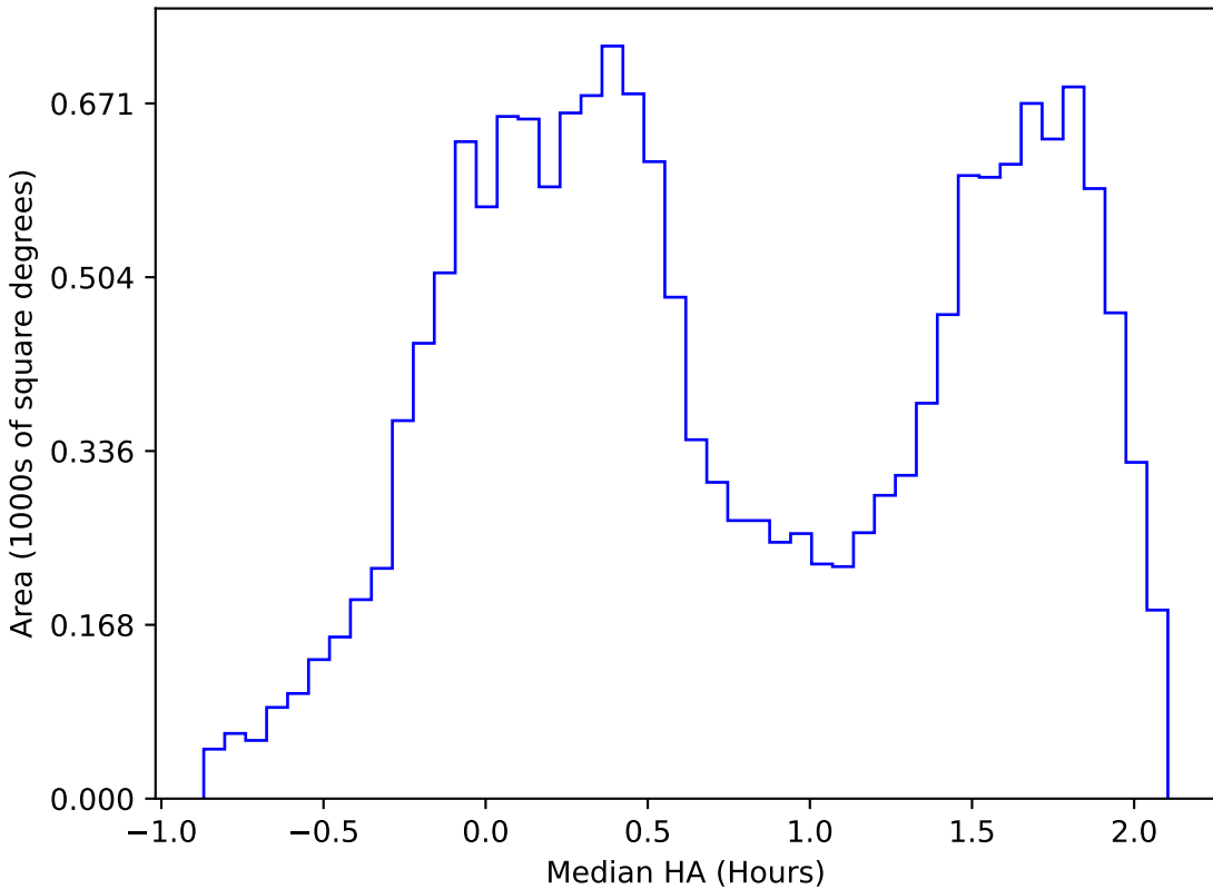
roll_pause_mjdp270_v3.4_10yrs WFD r band: Median HA
