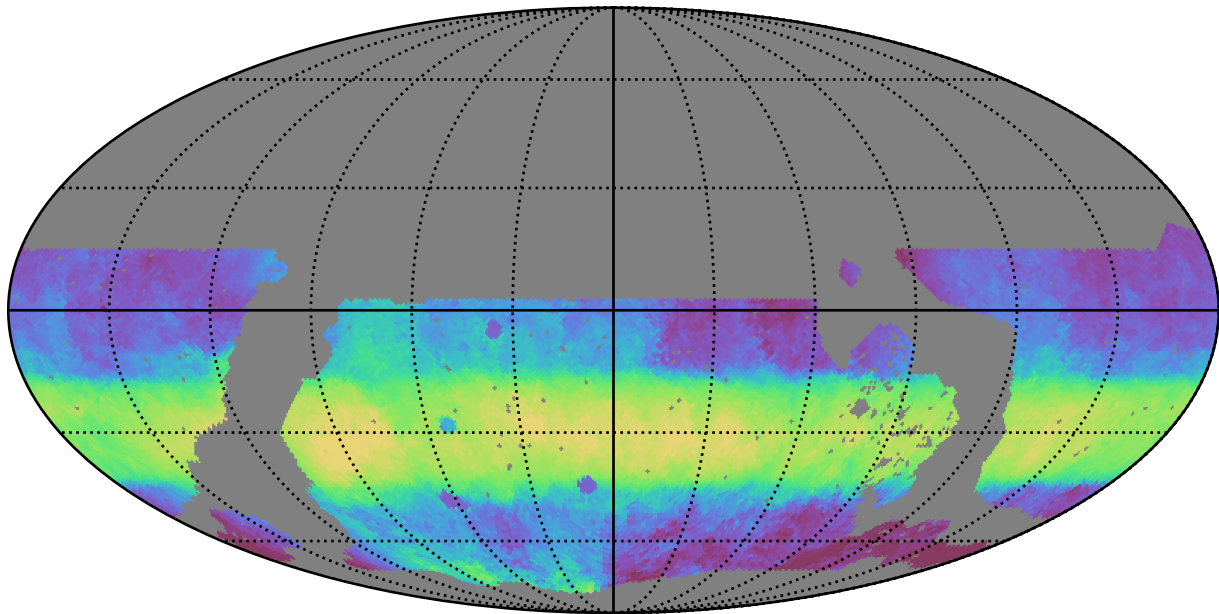
roll_pause_mjdp270_v3.4_10yrs WFD i band: Median HA
