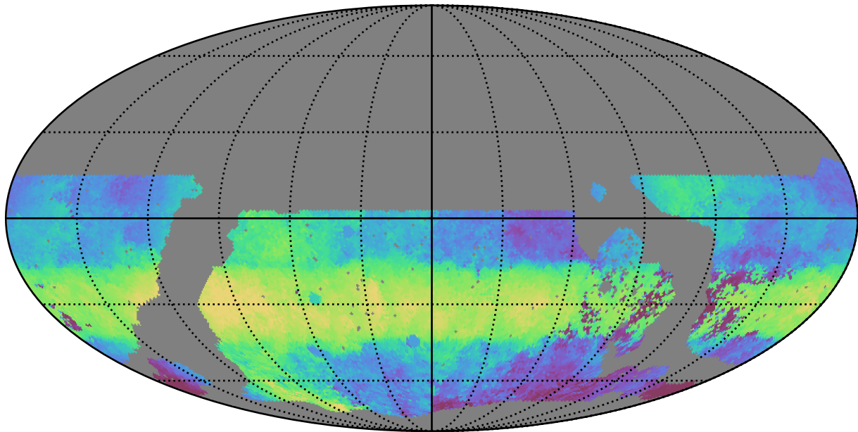
roll_pause_mjdp270_v3.4_10yrs WFD g band: Median HA
