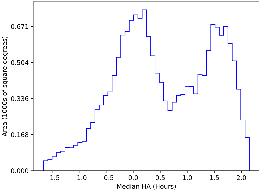
roll_pause_mjdp270_v3.4_10yrs WFD g band: Median HA
