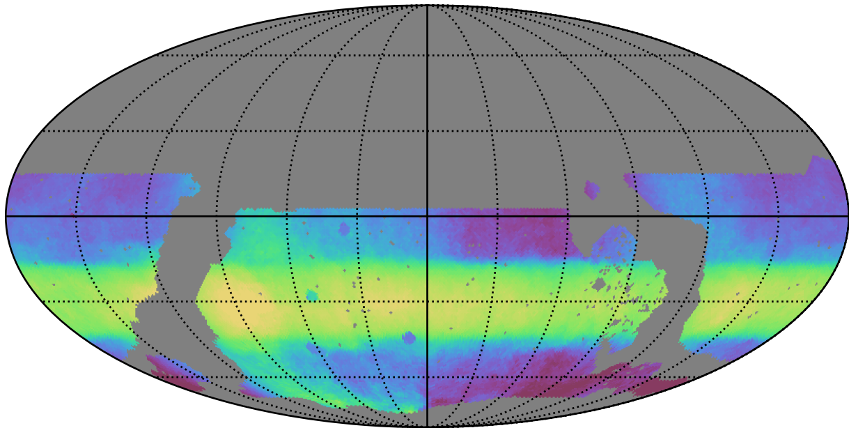
roll_pause_mjdp270_v3.4_10yrs WFD all bands: Median HA
