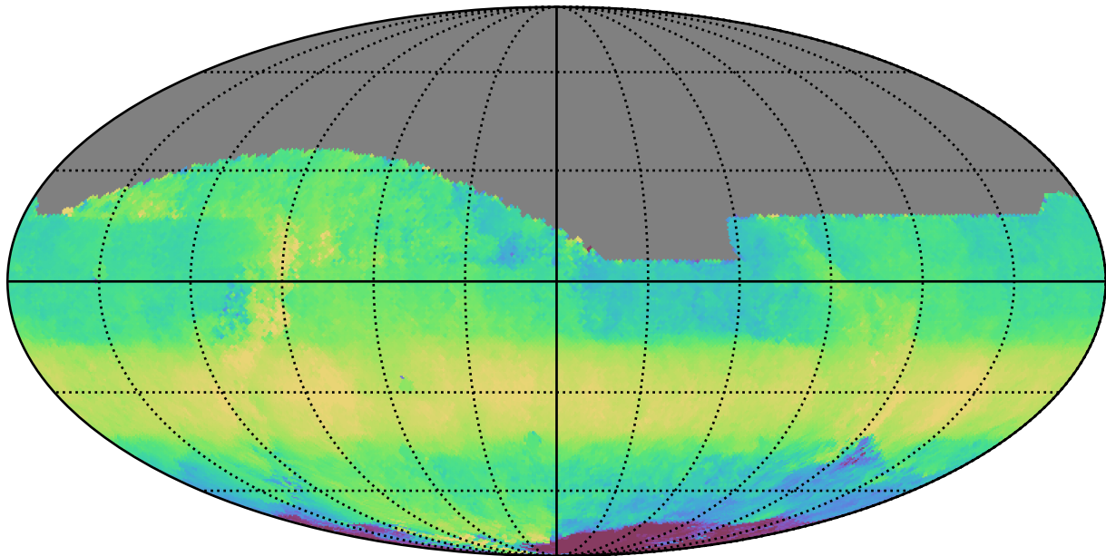
roll_pause_mjdp270_v3.4_10yrs All sky z band: Median HA
