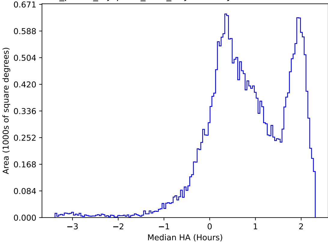
roll_pause_mjdp270_v3.4_10yrs All sky z band: Median HA
