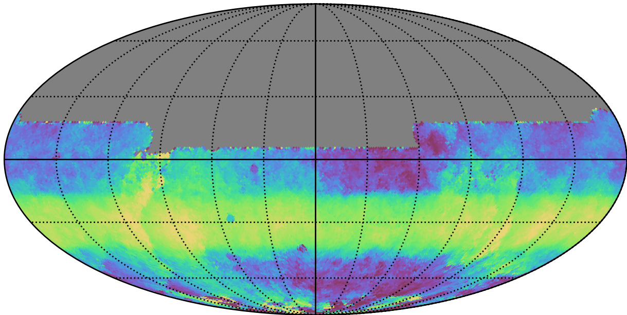
roll_pause_mjdp270_v3.4_10yrs All sky y band: Median HA
