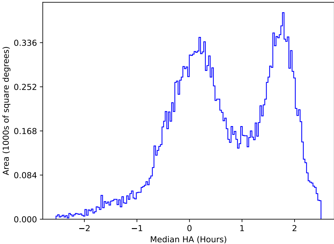
roll_pause_mjdp270_v3.4_10yrs All sky u band: Median HA
