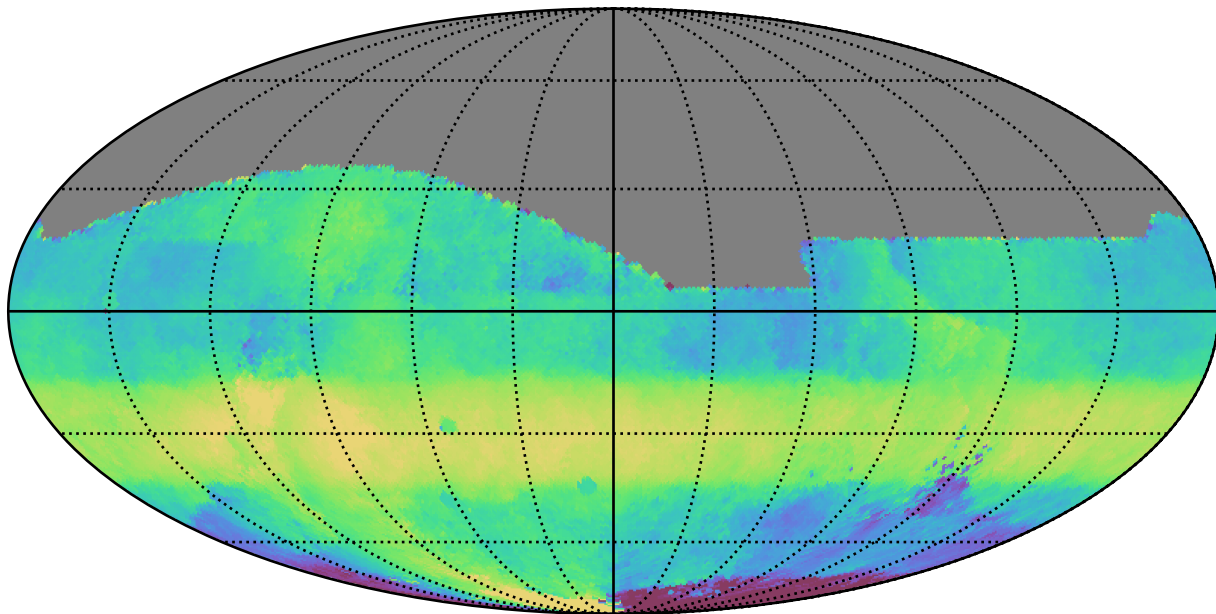
roll_pause_mjdp270_v3.4_10yrs All sky r band: Median HA
