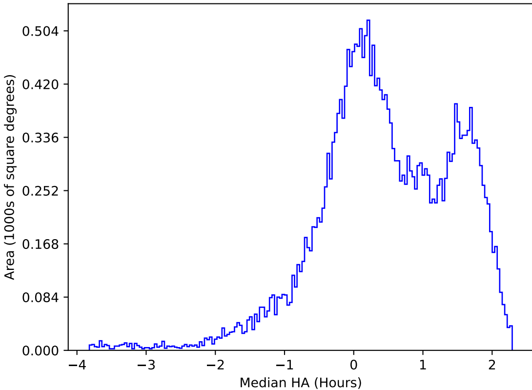
roll_pause_mjdp270_v3.4_10yrs All sky g band: Median HA
