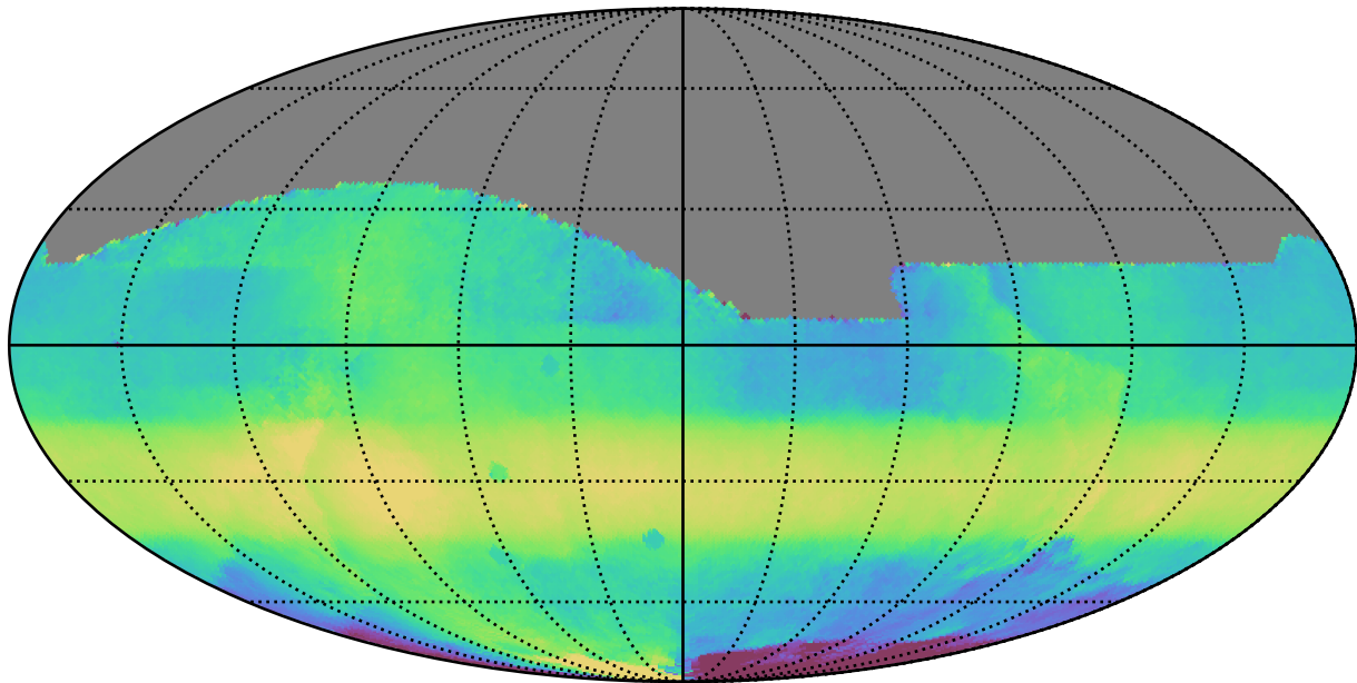
roll_pause_mjdp270_v3.4_10yrs All sky all bands: Median HA
