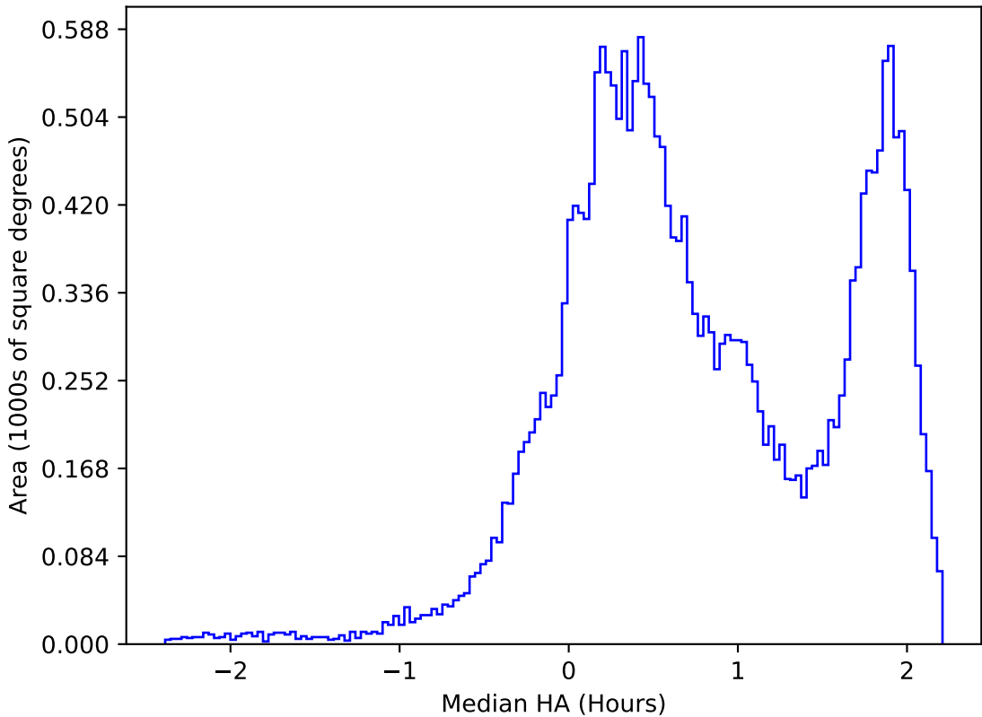
roll_pause_mjdp270_v3.4_10yrs All sky all bands: Median HA
