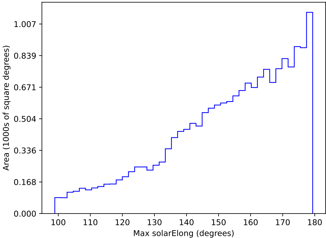
roll_pause_mjdp270_v3.4_10yrs WFD z band: Max solarElong
