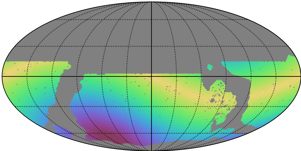
roll_pause_mjdp270_v3.4_10yrs WFD y band: Max solarElong
